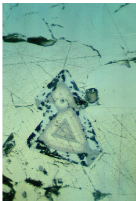
Figure 22. Zoned pyrite-siegenite-bravoite surrounded by galena. Hack 2 Mine, Field of view = 0.11 mm
