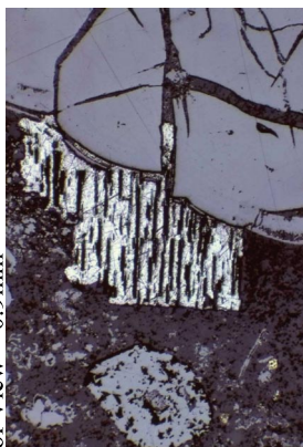
Figure 25. Later galena filling crack in uraninite, sphalerite to left of galena, Hack 2 Mine, Field of view = 1.0mm
