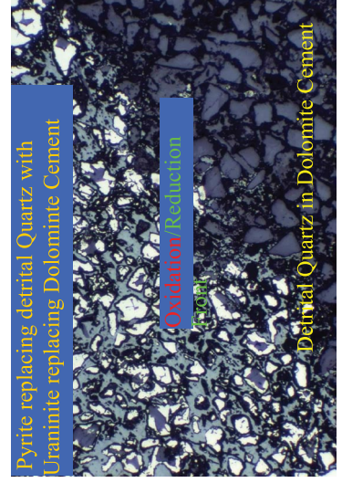
Figure 19. Reflected light photomicrograph with an oxidation/reduction front. Pigeon Mine
