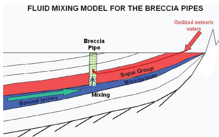
Figure 41. Fluid-mixing model for the breccia pipe ore genesis.
