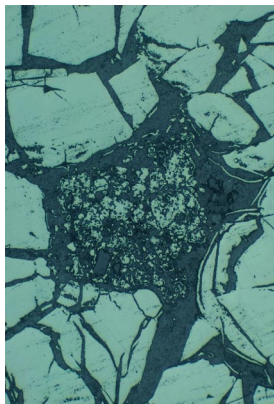
Figure 24. Uraninite-2 Stages: early stage later fractured and later wispy stage. Hack 2 Mine, FOV = 1.34mm
