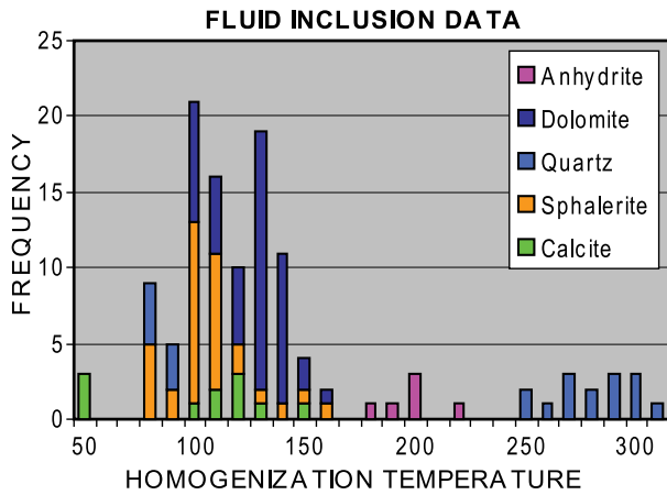
Figure 32. Homogenization temperatures for mineral phases associated with breccia-pipe ore. Each frequency represents a separate fluid inclusion. Temperatures below 80°C are from non-pipe calcite shown as a contrast. The high temperature quartz is believed to be from a late stage of silicification. Minerals related to ore forming processes precipitated from fluids with temperature between 80° and 173°C.
