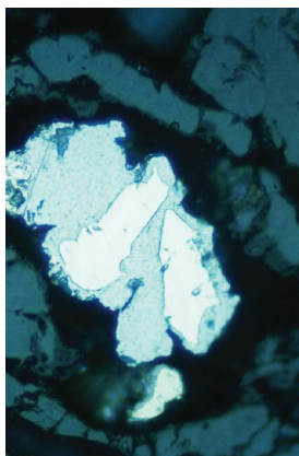
Figure 23. Gersdorffite in galena surrounded by uraninite, Hack 2 Mine, Field of view = 0.09mm
