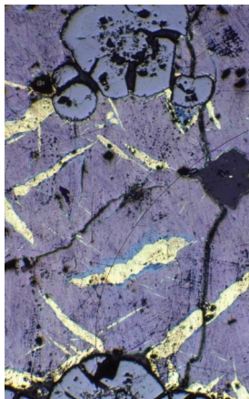
Figure 26. Uraninite with bornite, digenite, covellite, and chalcopyrite. Orphan Mine.
