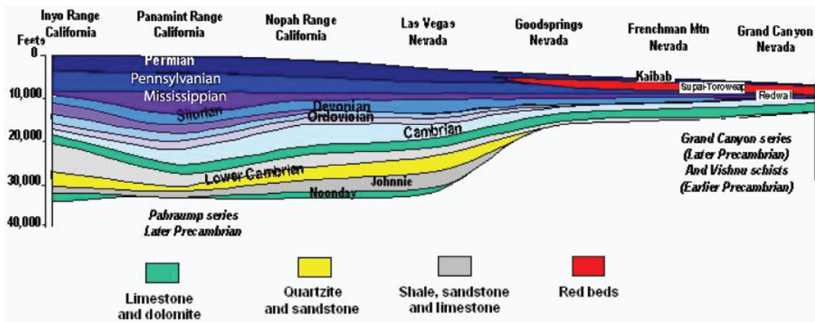
Figure 34. Cross section of Paleozoic miogeosyncline from the Grand Canyon to the Inyo Mountains, California. From P.B. King (1959; Fig. 77, p. 135).
