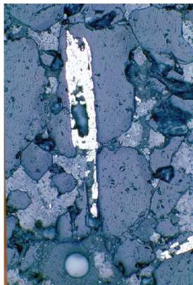
Figure 20. Pyrite after barite, Orphan Mine, Field of View = 0.25 mm
