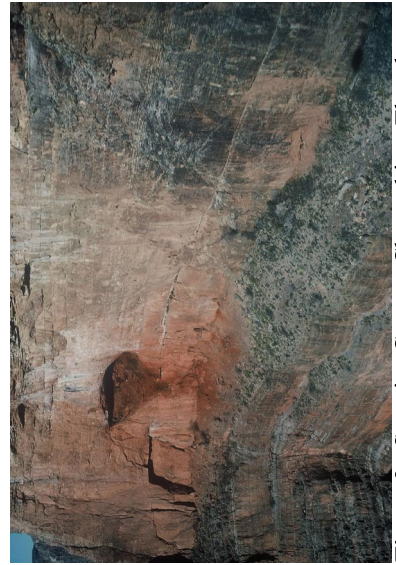
Figure 9. Surprise Canyon Channel in a Thunder Springs Cave
