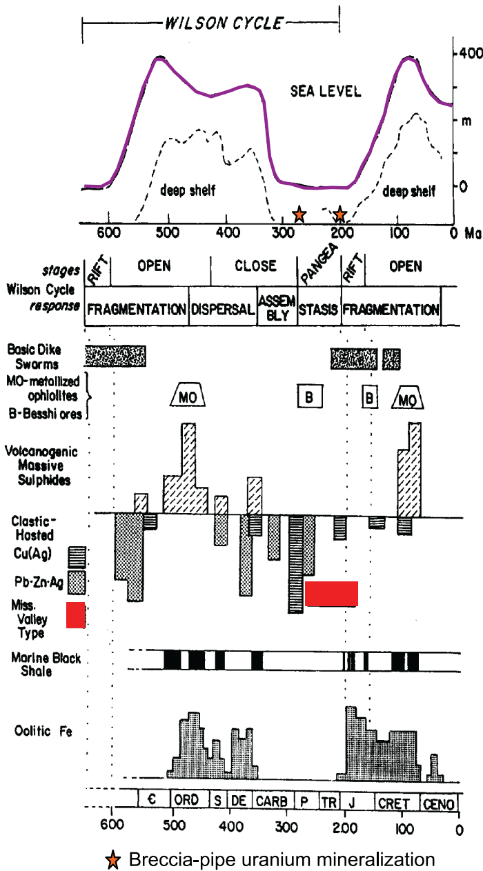
Figure 36. Wilson cycle stratabound ore relationships. MVT ore in red and breccia-pipe uranium mineralization shown with red stars. Modified from Tittley (1993).
