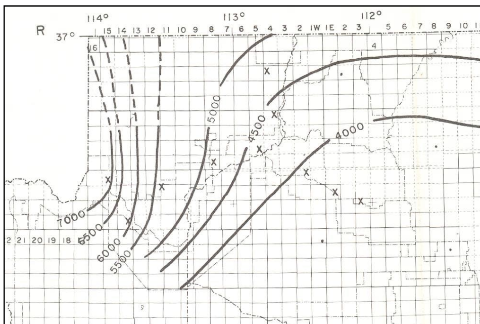
Figure 35 (right). Isopach map, in feet, of all Paleozoic strata in northwestern Arizona. Westward thickening toward the miogeocline is apparent, as is the Paleozoic shelf environment of the breccia pipe regions (from McKee, 1951).
