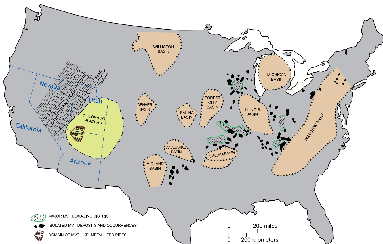
Figure 38. Mid-continent MVT districts and basins, modified from Cathles and Smith (1983).
