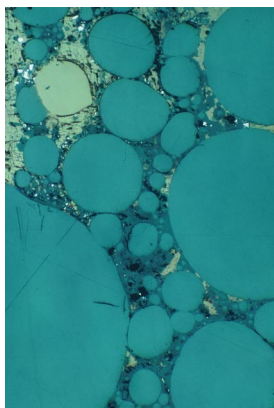
Figure 27. Bitumen Balls, Pigeon Mine, Field of view = 1.29mm
