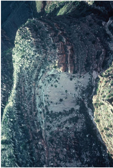
Figure 12. The Ridenour mine, located on the Hualapai Reservation, has been mined intermittently for copper since the 1870's. All that remains of this pipe at the level of the Esplanade Sandstone is one-third of the ring-fracture zone. Samples with uranium concentrations of 3,000 ppm and vanadium concentrations of 4% are present on the outcrop surface where the bleached Esplanade Sandstone has been dissected by the canyon.
