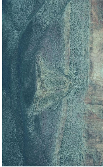
Figure 15. Pipes exposed from the canyon wall upward to the overlying plateau are rare. Here at pipe #226 (location shown in Wenrich and others, 1996), the pipe exposure in the canyon wall is overlain by a shallow structural basin with concentrically inward-dipping beds.
