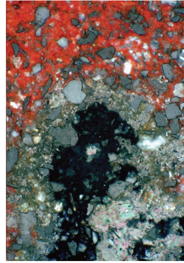
Figure 18. Transmitted light photomicrograph of Hematite + Uraninite, Pigeon Mine
