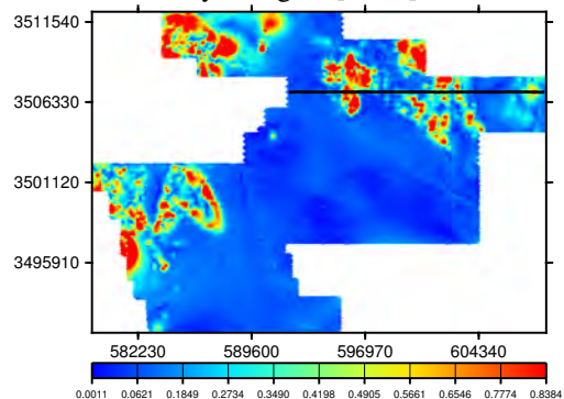
Analytic Signal [nT/m]
