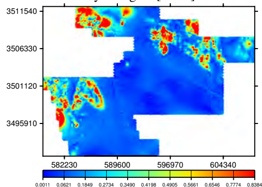
Analytic Signal [nT/m]
